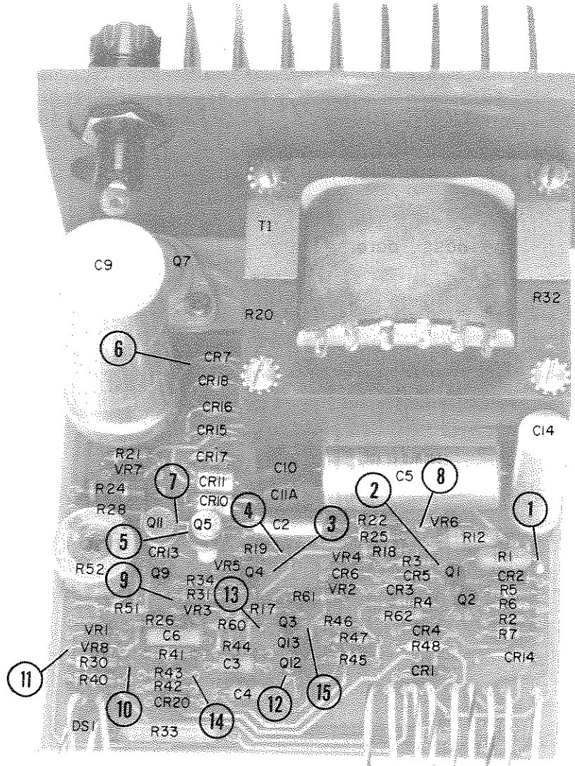
Figure A-1. Model 6216A, Components Location Diagram
